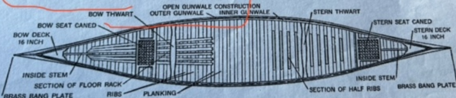
DIAGRAM of the "Old Town Canoe"
